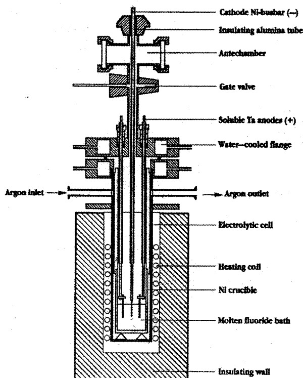
Fig. 1. Molten salt electrolytic cell.
