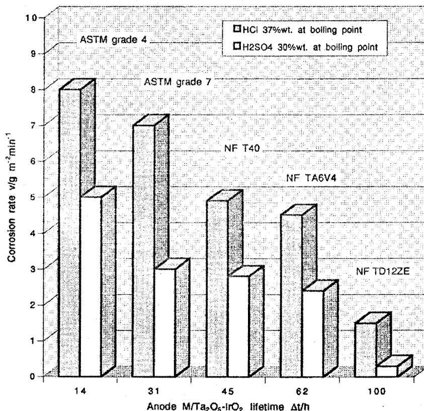
Fig. 2. Correlation between anode lifetime and corrosion rates in hydrochloric and sulfuric acids (anodes have a surface mass density of IrO 2 in the range of 15–17 g m -2 ).
